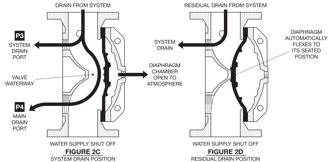
FIGURE 2 DV-5 DELUGE VALVE SET AND OPEN POSITIONS
