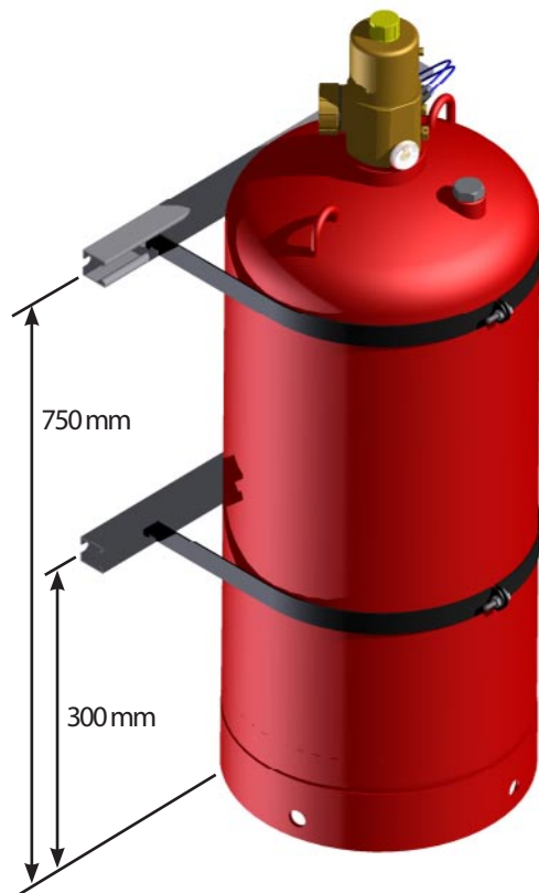
Figure 48 - Container Strap Location (106L Example)
